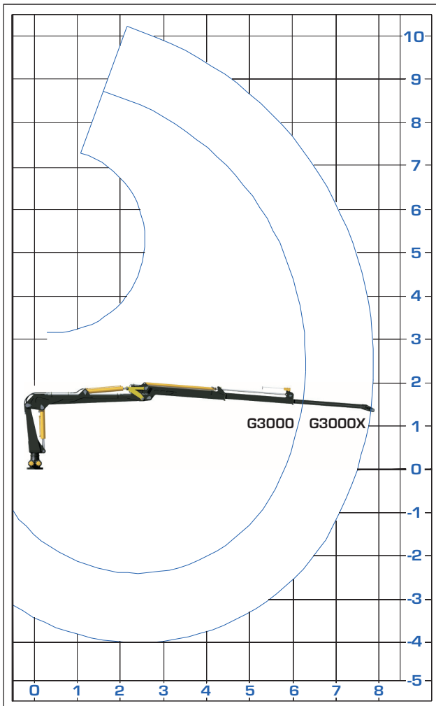
Load diagram
