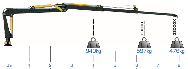
Load diagram
